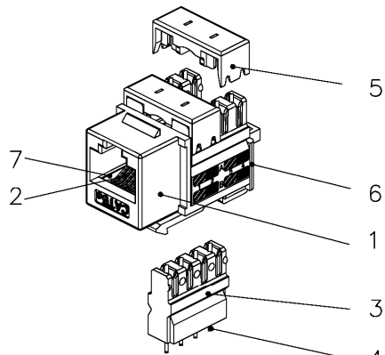
KRONE 45-110 DUAL IDC
