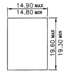
Single Panel-Latch Clearance Panel Thickness 0.062 inch
