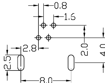
P. C. B. LAYOUT (Tolerance: ±0.10)
