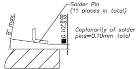
View of Coplanarity
