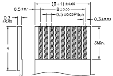
Applicable FPC
