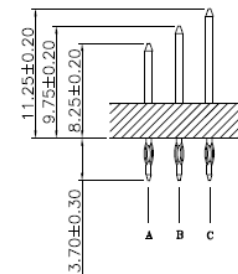
CONTACT LAYOUT
