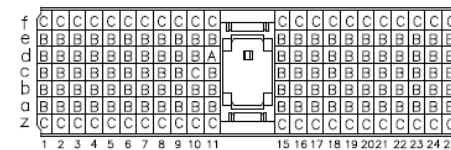
CONTACT LAYOUT
