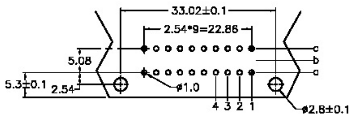
P.C. Board Layout (Tolerance: ±0.05)
