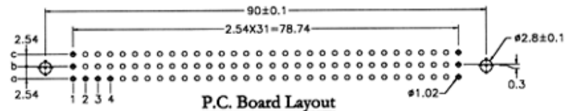
P.C. Board Layout
