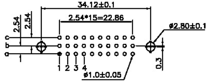
P.C. Board Layout (Tolerance:±0.05)
