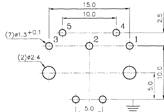
MOUNTING HOLE (TOP VIEW)
