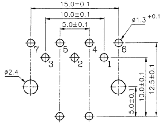
MOUNTING HOLE (TOP VIEW)
