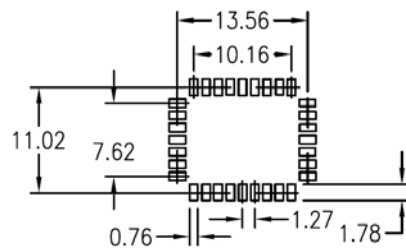
RENNMENDED P.C.B PAD LAYOUT
