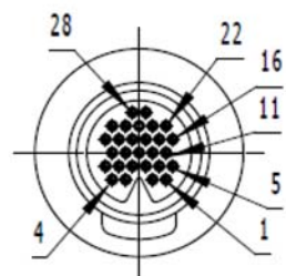
A direction insert arrangement
