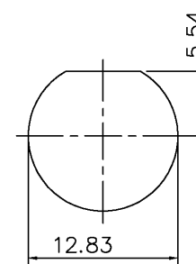
RECOMMENDED MOUNTING HOLE MAXIMUM PANEL THICKNESS: 5.5MM
