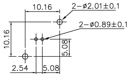
RECOMMENDED PCB BOARD LAYOUT WITHOUT MOUNTING POSTS
