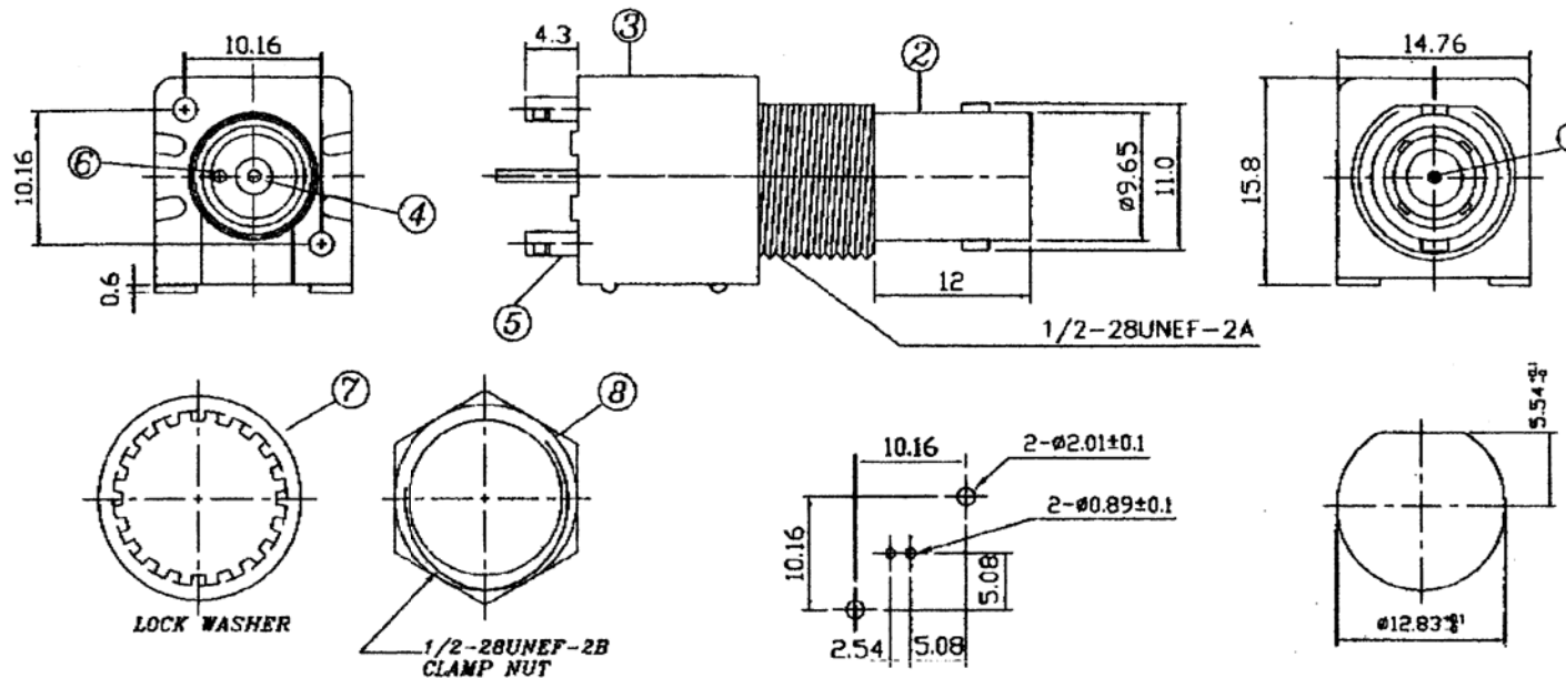
RECOMMENDED PC BOARD LAYOUT WITHOUT MOUNTING POSTS
