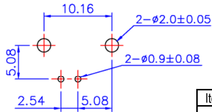
RECOMMENDED PC BOARD LAYOUT WITHOUT MOUNTING POSTS
