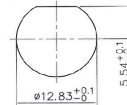
RECOMMENDED MOUNTING HOLE MAXIMUM PANEL THICKNESS: 5.5MM
