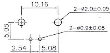
RECOMMENDED PC BOARD LAYOUT WITHOUT MOUNTING POSTS
