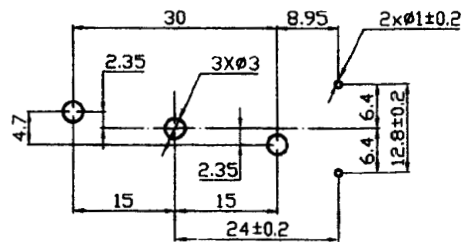
PCB/MOUNTING LAYOUT
