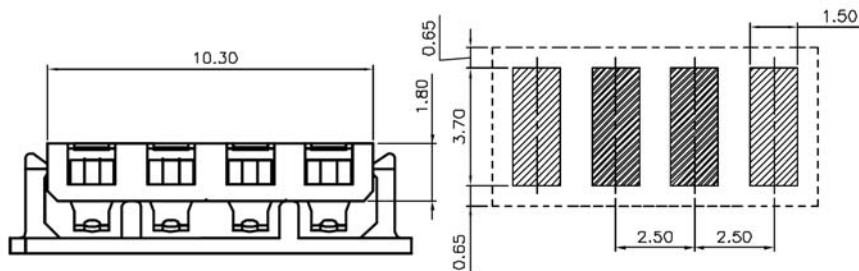
P.C BOARD LAYOUT (TOLERANCE: \pm 0.15\text{mm} ) AS VIEW FORM COMPONENT SIDE
