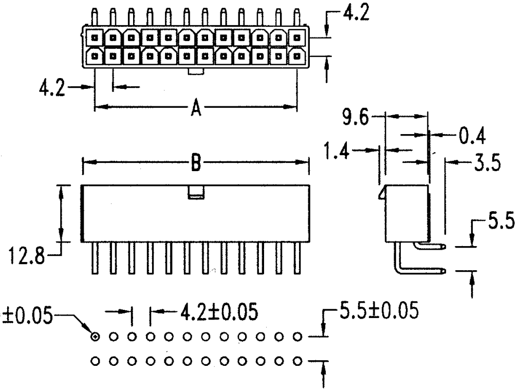
PC Board Hole Layout and Dimensions
