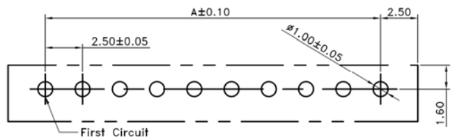
Recommended PCB Layout (Top View)
