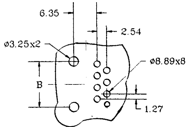
LAYOUT/TOP VIEW
