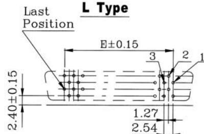
Standard PC Board Layout
