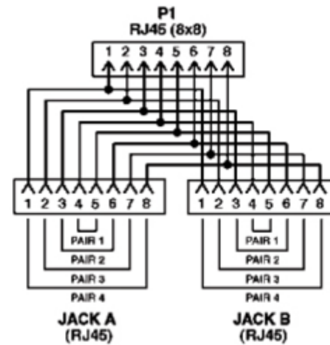
Pin Out Chart
