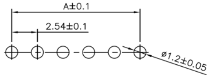
Recommand PCB Layout
