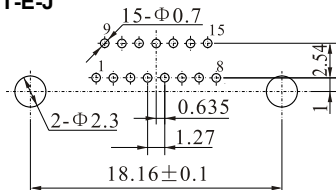
DSM15-FT-E-J
