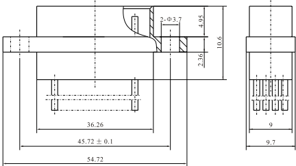
DSM100-FT
