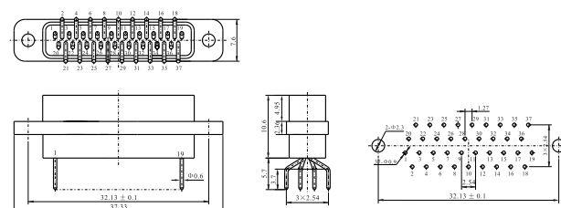
DSM37-FT-R
