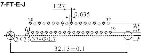
DSM37-FT-E-J
